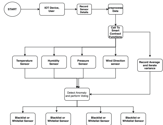
Fig. 3. Flow chart for the Anomaly Detection Mechanism
